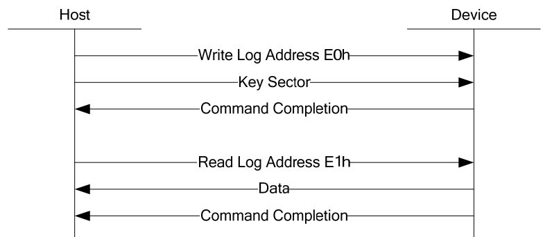
Figure 15 – Example sequence for reading data using an SCT command with no background activity
