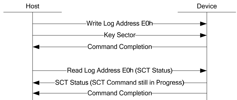
Figure 16 – Example Sequence for a non-datan SCT command with no background activity
