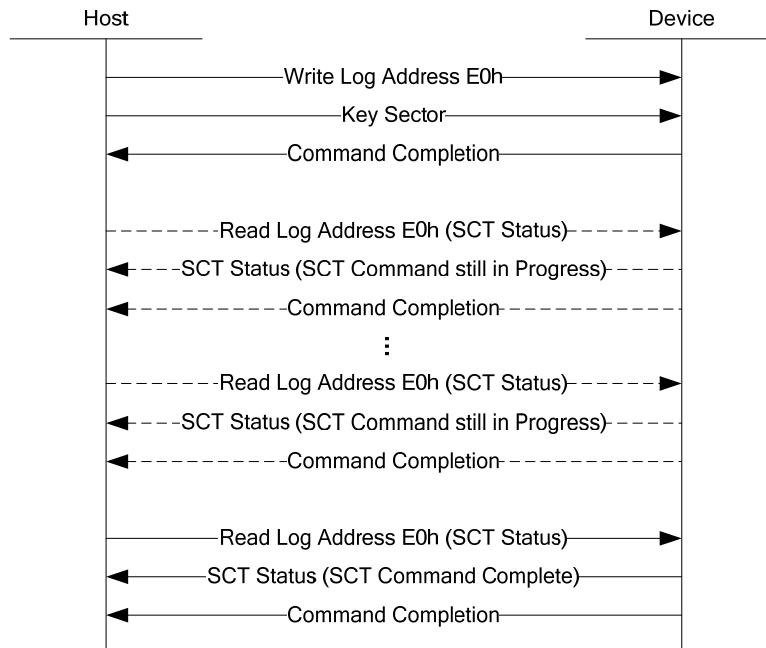
Figure 18 – Example sequence for a non-datan SCT command with background activity
