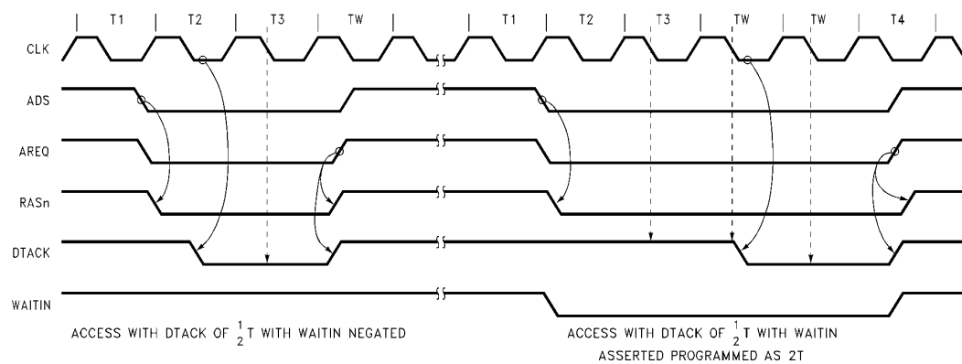
FIGURE 24a. \overline{WAITIN} Example ( \overline{DTACK} is Sampled at the "T3" Falling Clock Edge)
