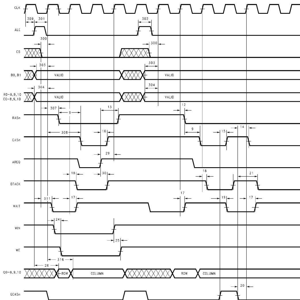
FIGURE 40. 300: Mode 0 Timing
