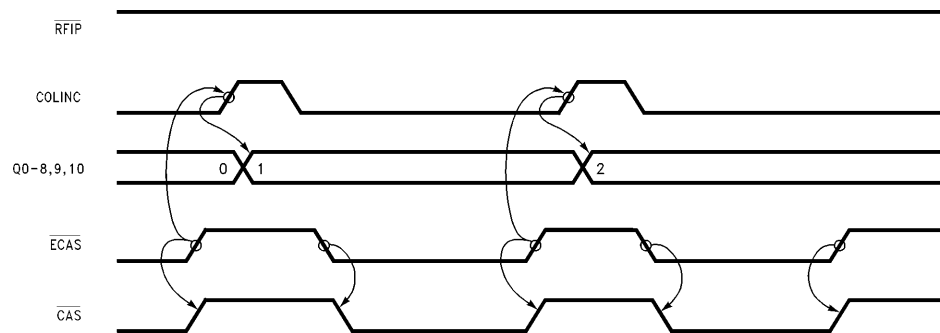
FIGURE 10. Column Increment
