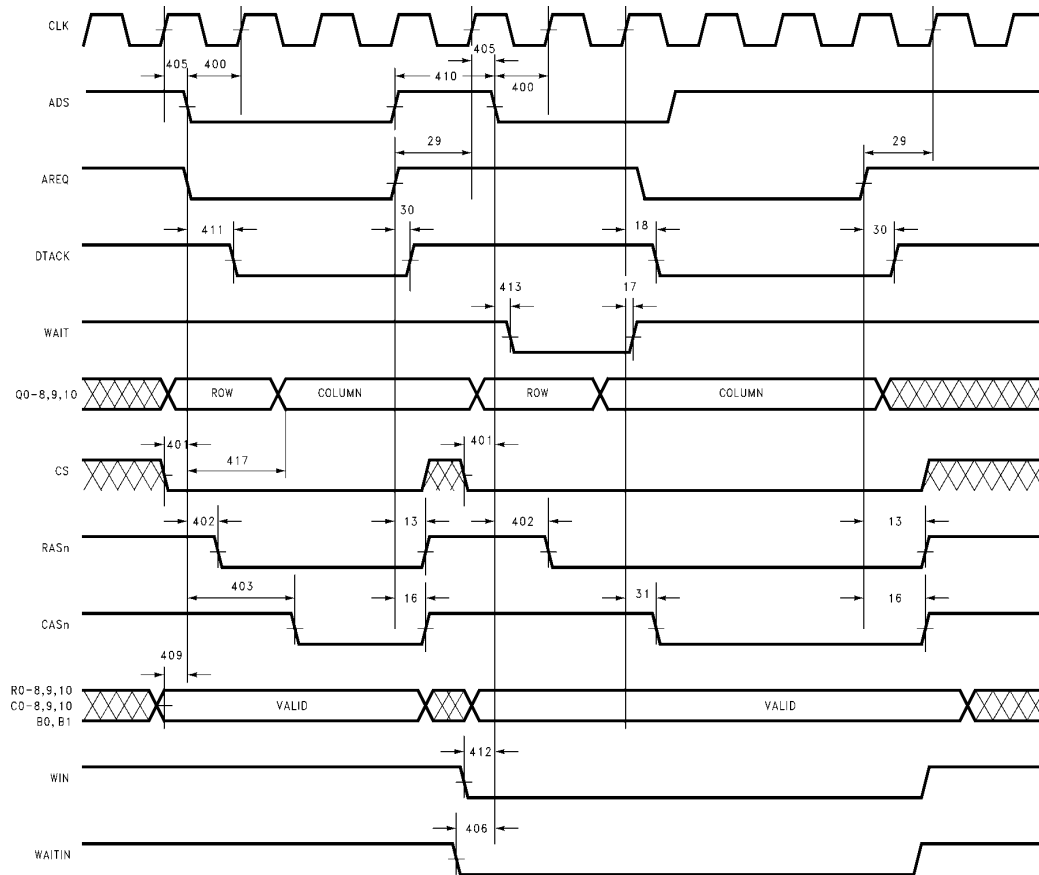
FIGURE 42. 400: Mode 1 Timing
