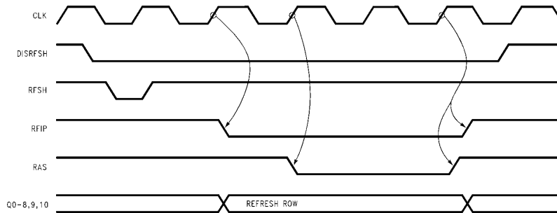
FIGURE 14a. Single External Refreshes (2 Periods of \overline{\text{RAS}} Low during Refresh Programmed)
