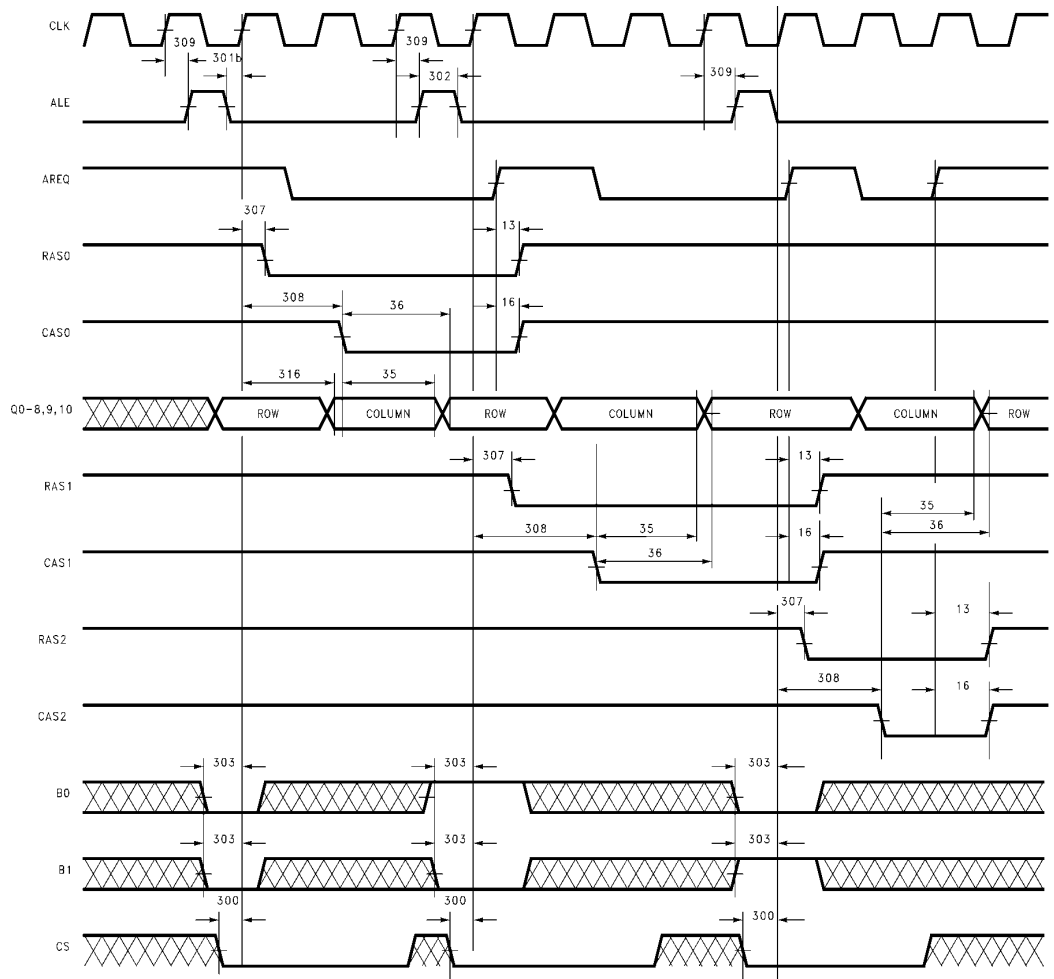
FIGURE 41. 300: Mode 0 Interleaving
