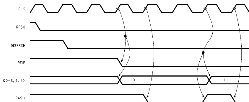
FIGURE 20b. Clearing the Refresh Counter during Burst
