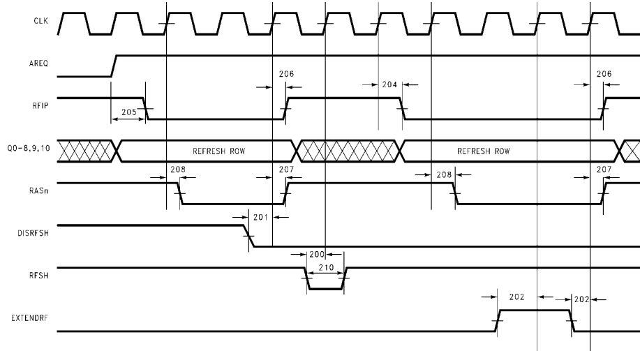
FIGURE 39. 200: Refresh Timing
