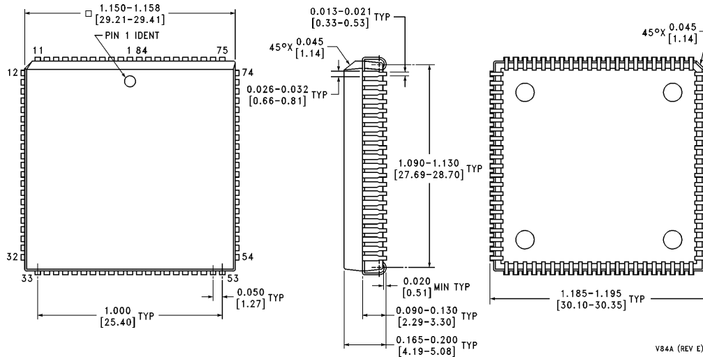
Plastic Chip Carrier (V) Order Number DP8422V-33 or DP84T22-25 NS Package Number V84A
